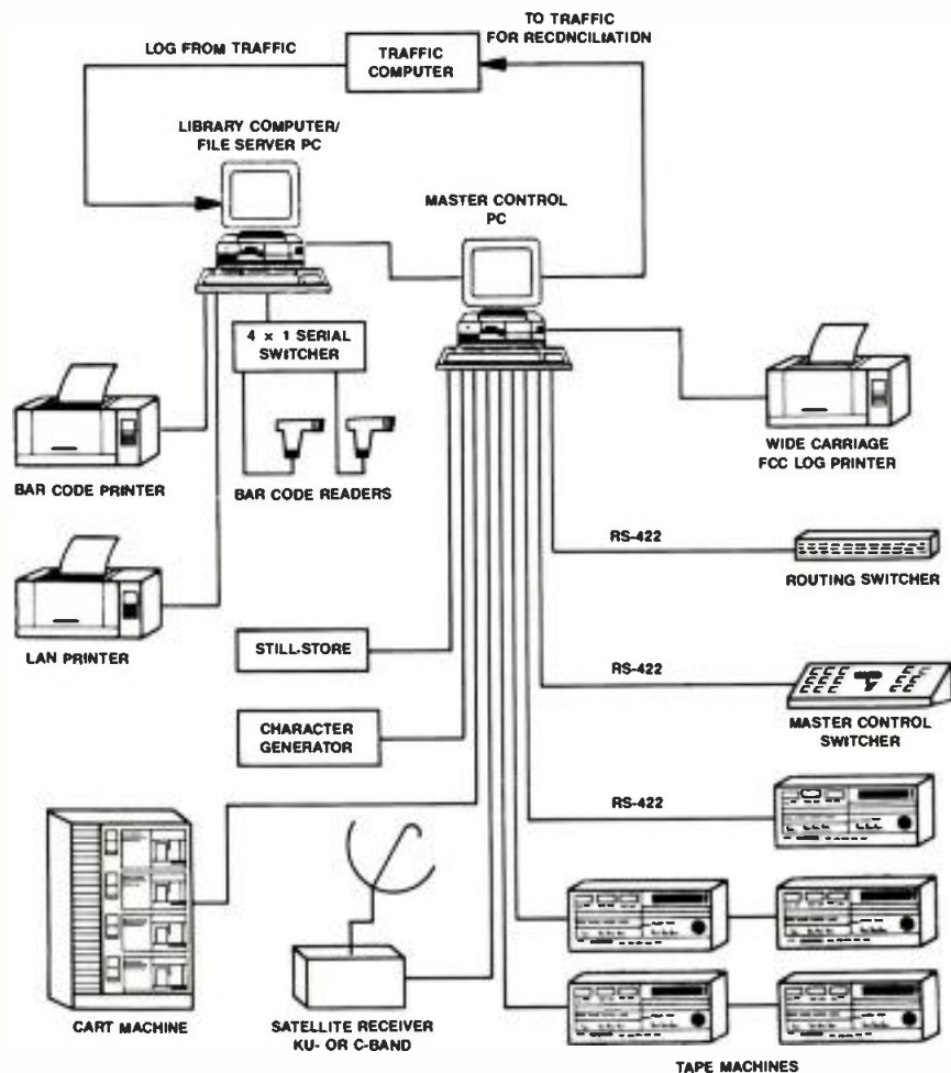
Figure 1. In this PC-based automation system the master control computer controls the on-air and recording tasks while following the electronic log provided by the traffic computer, and reporting back the as-run log for reconciliation. (Courtesy of Columbine Systems.)
