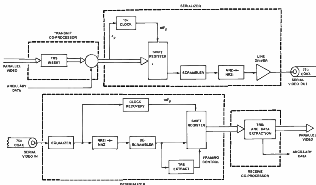
Figure 1. A block diagram of a typical serializer and deserializer pair.
