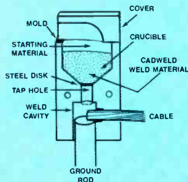
Figure 1. The Cadweld welding process ignites metal powders in a graphite crucible to meld metals with a molecular bond. User applies spark with flint lighter.
