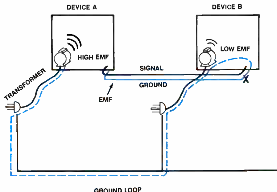
Figure 2. A ground loop when stray currents flow between two devices with different potentials along the ground system. Grounding only at the low-impedance end can prevent formation of ground loops.
