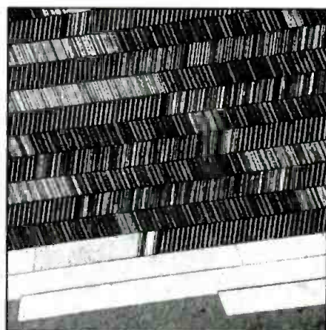
Digital video formats D-1 (left) and D-2 (right) are compared at 100 \times magnification. Note D-1's guardbands and uniform azimuth relationship, whereas D-2's alternating azimuth recording allows the elimination of guardbands, providing greater density. D-2's helical tracks actually overlap slightly, as shown at bottom right. Effective track widths are nearly identical between formats, but D-2's linear tape speed (5.18ips) is less than half of D-1's (11.3ips). (Courtesy of 3M.)
