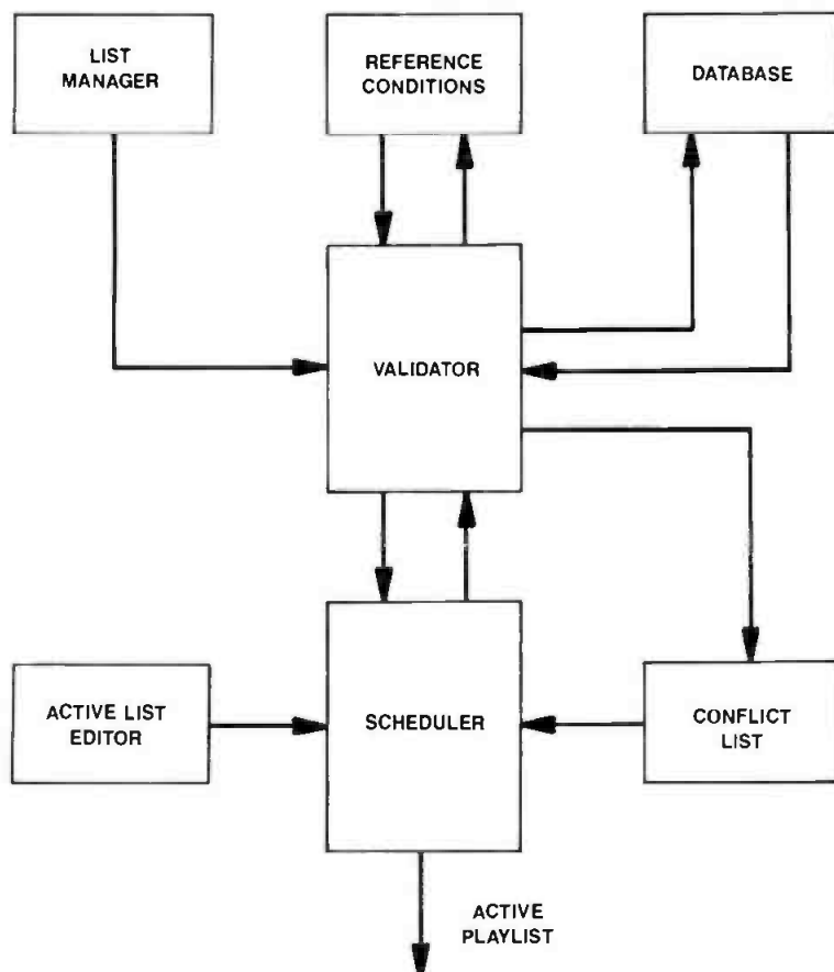
Figure 3. Flow diagram depicting the major elements of the AutoResolve system.
