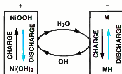
Figure 1. The reactions involved in nickel-metal hydride battery chemistry.
