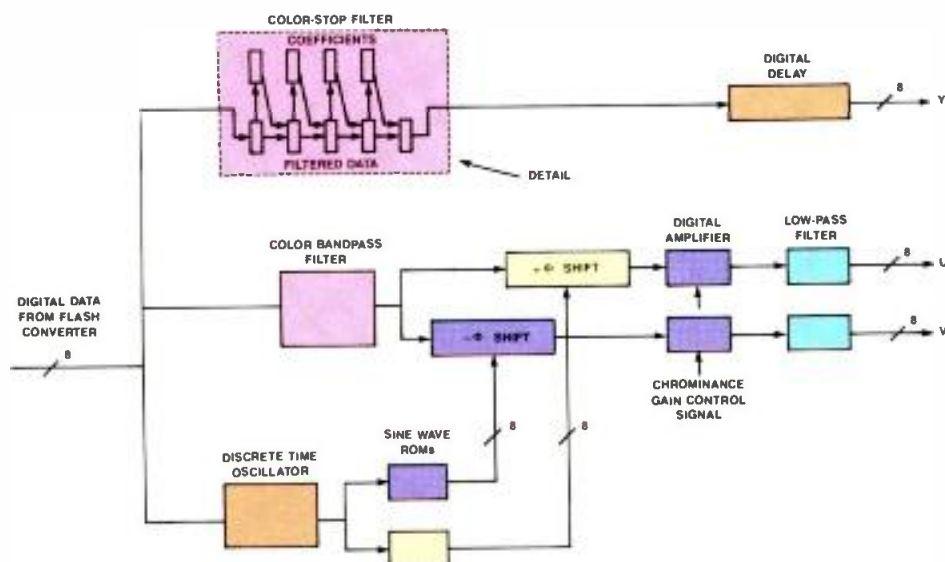
Figure 1. Internal block diagram of a digital multistandard decoder chip. The detailed section illustrates the operation of the filters. Signals step through shift registers accompanied by successive coefficient multiplication stages.
