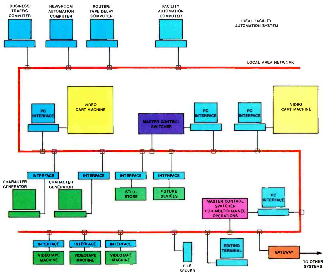
Figure 2. In a facility-wide automation system, all the automation islands become subsystems that share the station's production resources. The LAN enables the assigning and reassigning of devices.
