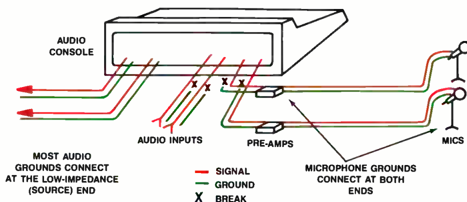
Figure 1. Audio grounds are nearly always connected at the low-impedance end, which is the source. This facilitates draining interfering signal to ground. The one exception is microphone pre-amplifiers, which are grounded to the pre-amplifier chassis because of the low ( -60\text{dB} ) mic levels.
