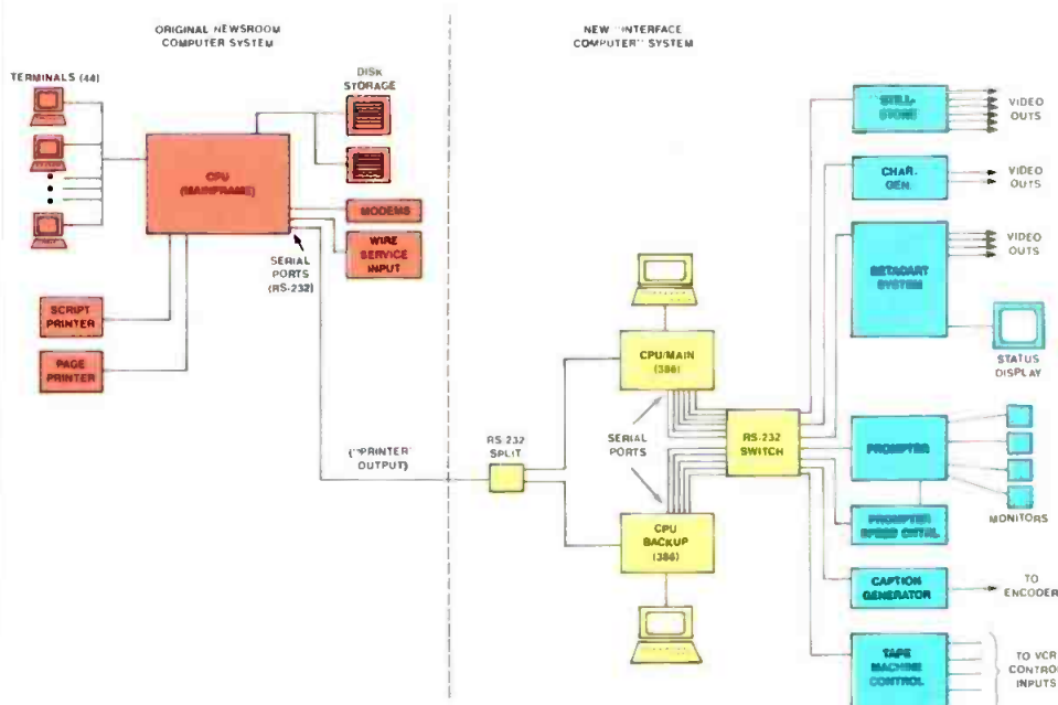
Figure 1. Basic block diagram of integrated newsroom computer system at WBNS-TV. Original newsroom system is at left, with retrofitted "interface computer" at right, adding automated device control. An RS-232 "printer" interface connects the two systems. Software running on 386 interface computers translates embedded control codes in news scripts to machine control data.
