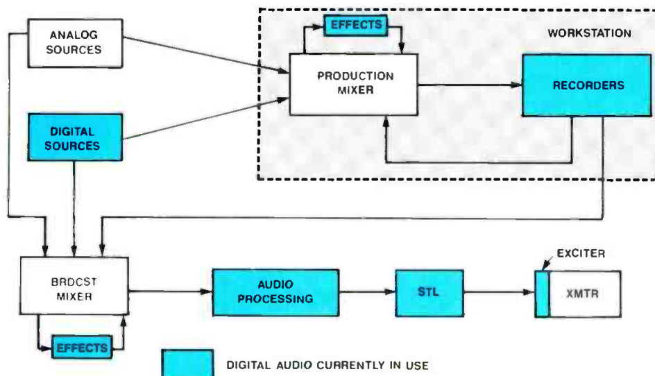
Figure 1. A block diagram of a typical radio station's signal path, showing components where today's digital audio technology is generally advantageous.
